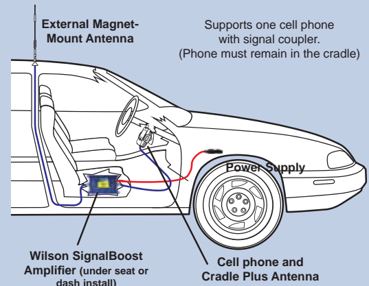
SignalBoost Amplifier Kit - Part # 811214
